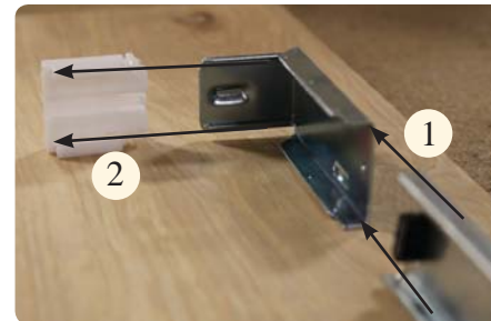
Temporarily place the back of the large drawer box slide into the mounting brackets as shown
